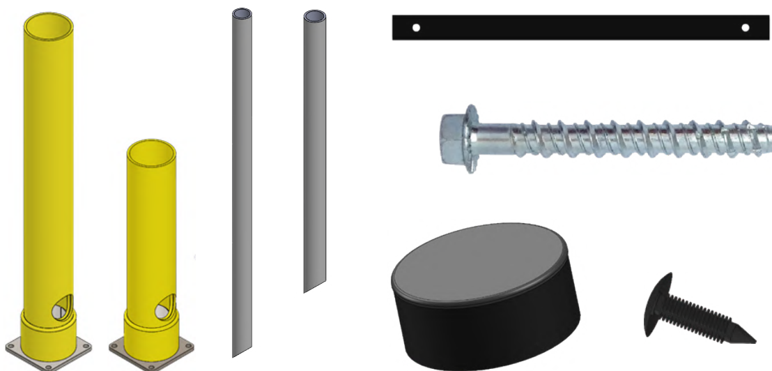
Figure 1. The BRD125 barrier components (list from left to right): finite post (1 pc. larger and 1 pc. smaller) with blind mounting holes, fixing pipes, section element (1 pcs), self-tapping anchor, post caps, screws.
