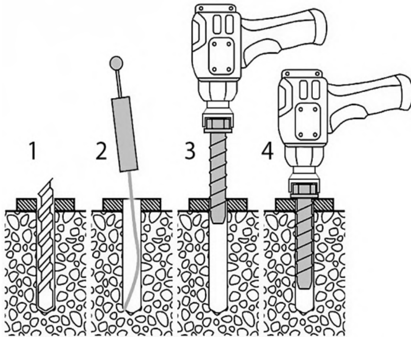
Figure 7. Barrier fixing
