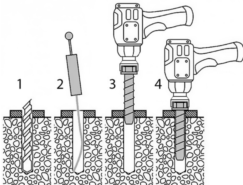
Figure 8. Barrier fixing
