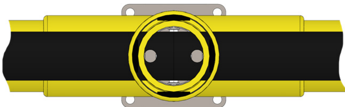
Figure 7. The proper arrangement of two adjacent sections inside connecting post (top view).
